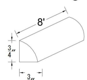
Quarter Round Molding
