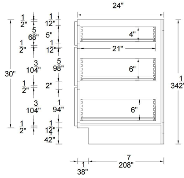
kitchen 3 drawers base standard
